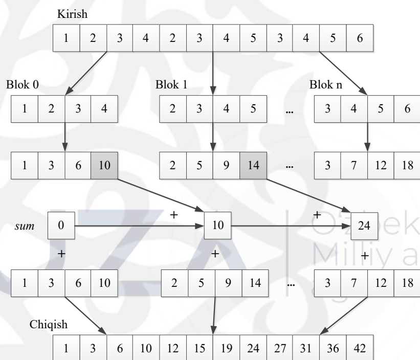
4-rasm. Parallel o'rtacha filtrlash algoritmi ( n = 12 , m = 4 ).
